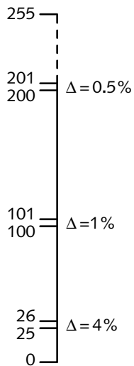
Figure 6.2 Fixed-point linear-light coding.
